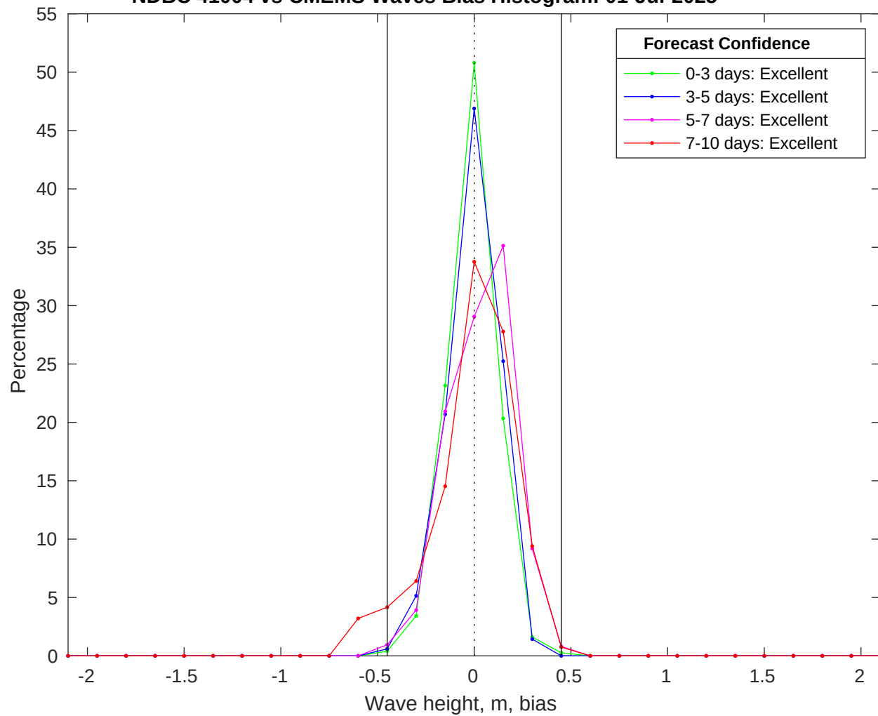
NDBC 41004 vs CMEMS Waves Bias Histogram: 01-Jul-2025
