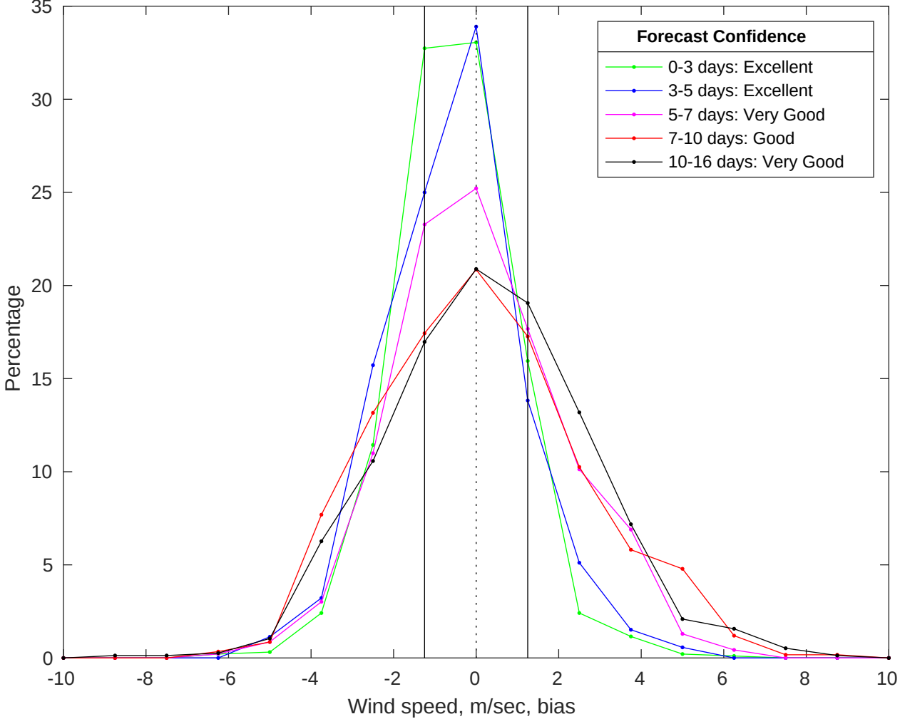
NDBC 41004 vs GFS Winds Bias Histogram: 01-Jul-2025
