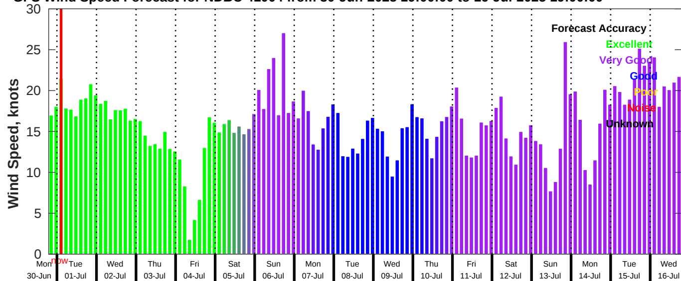
GFS Wind Speed Forecast for NDBC 41004 from 30-Jun-2025 19:00:00 to 16-Jul-2025 19:00:00
