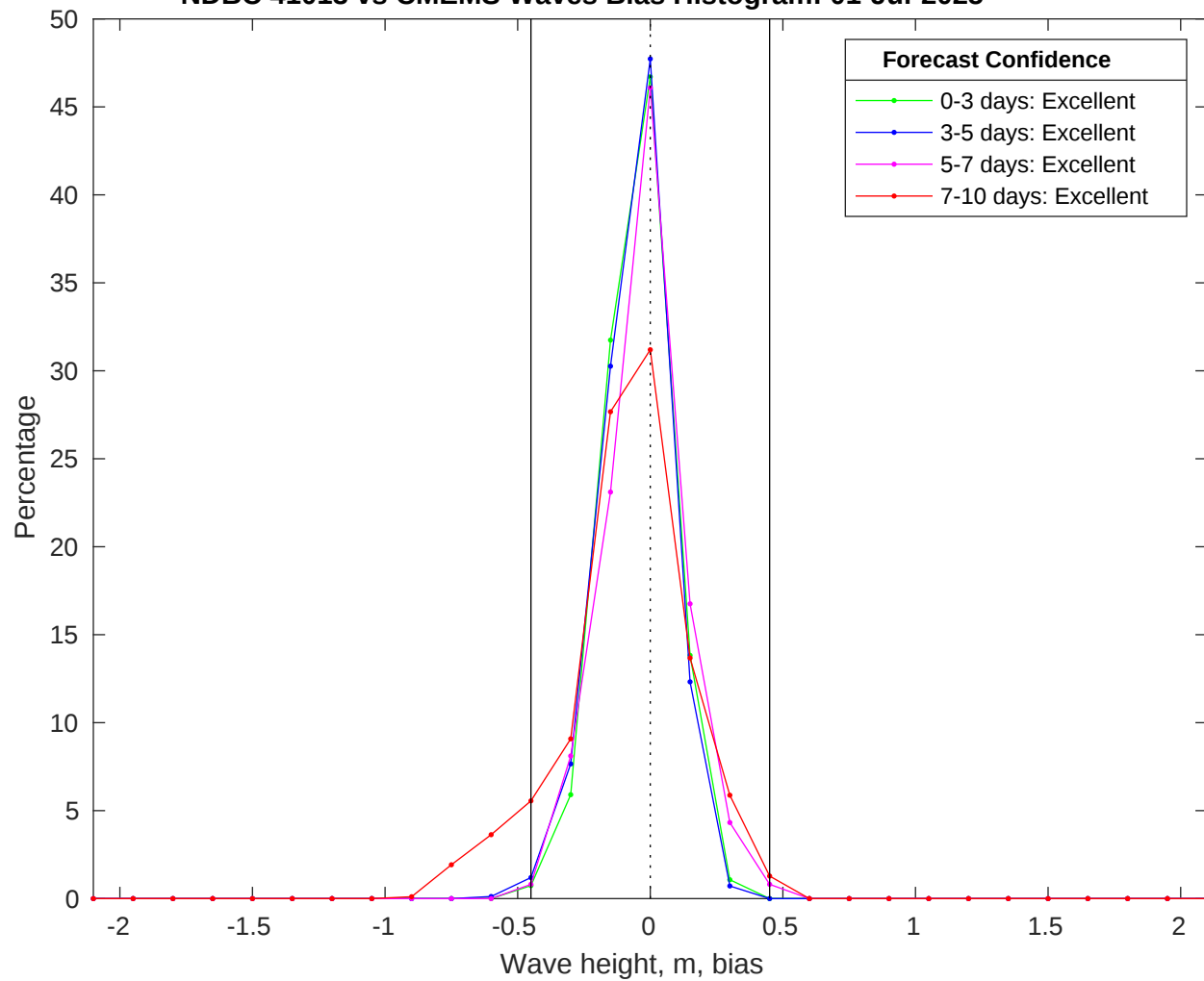
NDBC 41013 vs CMEMS Waves Bias Histogram: 01-Jul-2025
