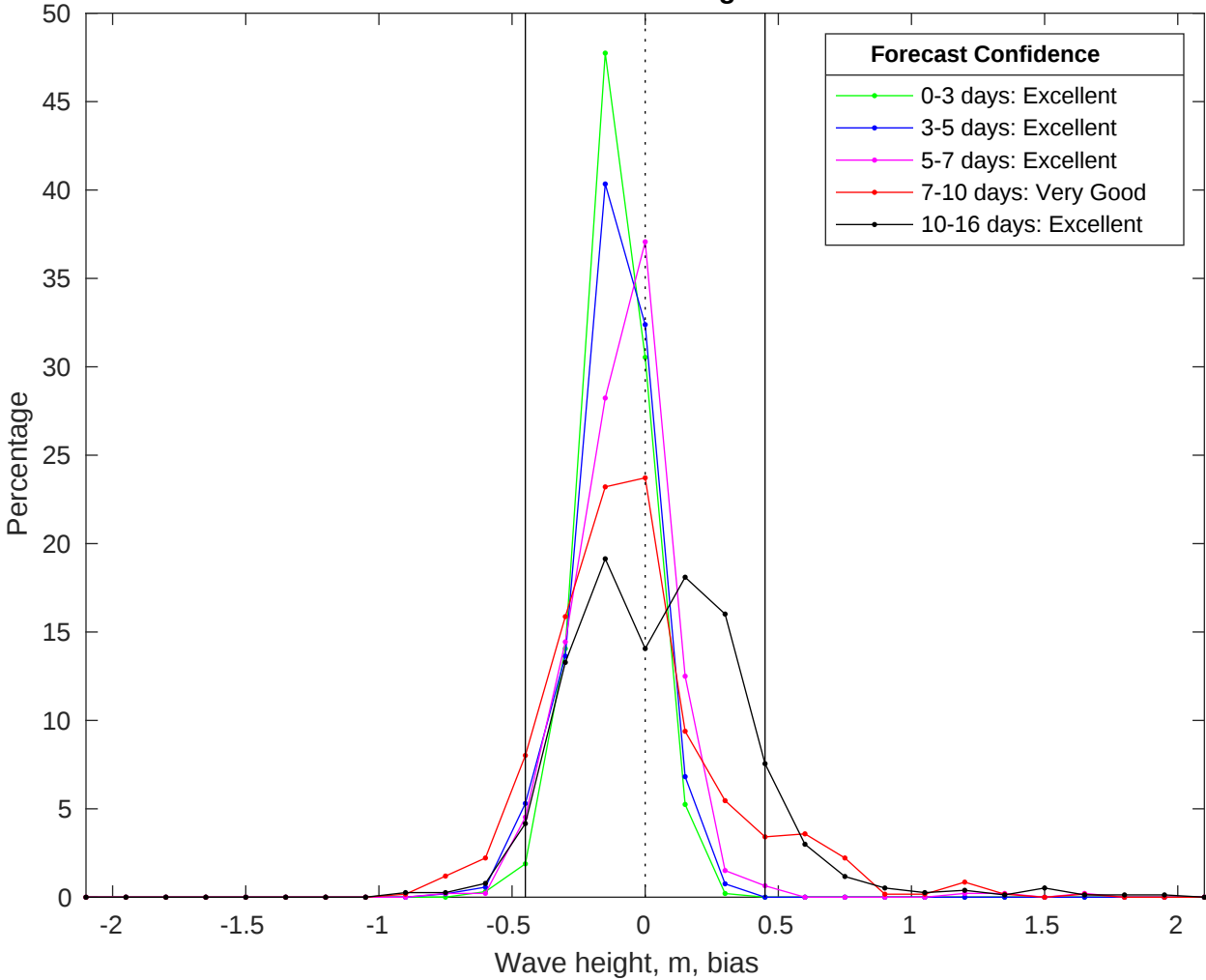
NDBC 41013 vs GFS Waves Bias Histogram: 01-Jul-2025
