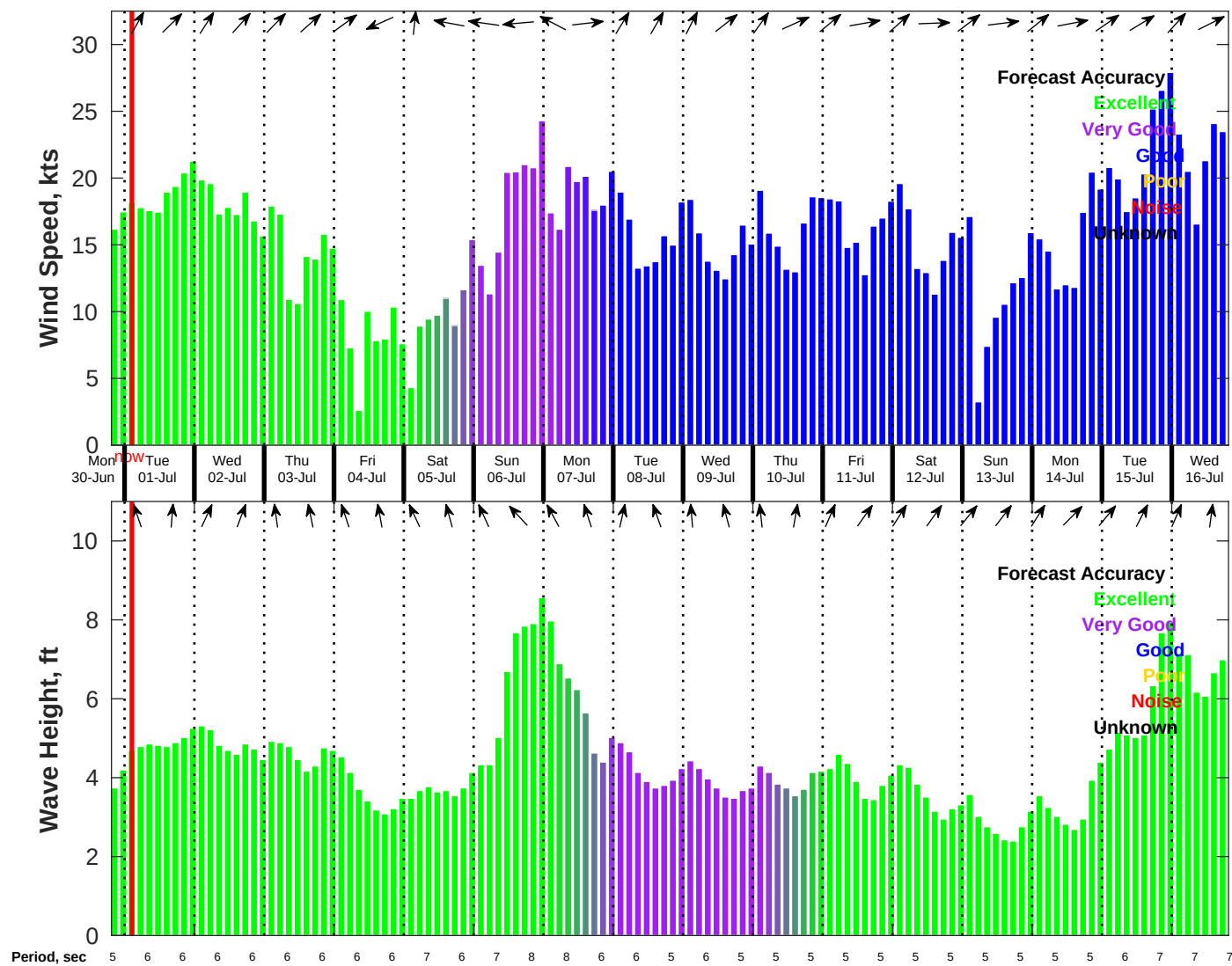
Wind & Wave Forecast for NDBC 41013 from 30-Jun-2025 19:00:00 to 16-Jul-2025 19:00:00
