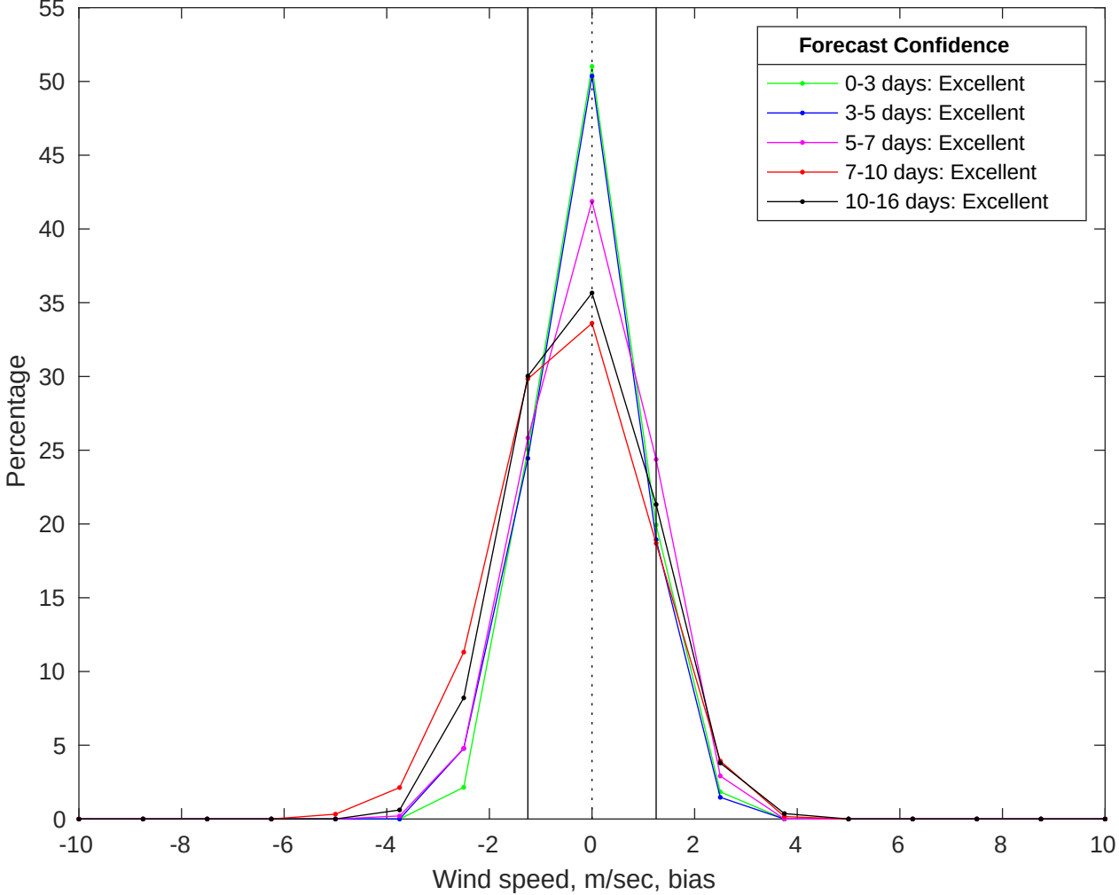
NDBC 41040 vs GFS Winds Bias Histogram: 01-Jul-2025
