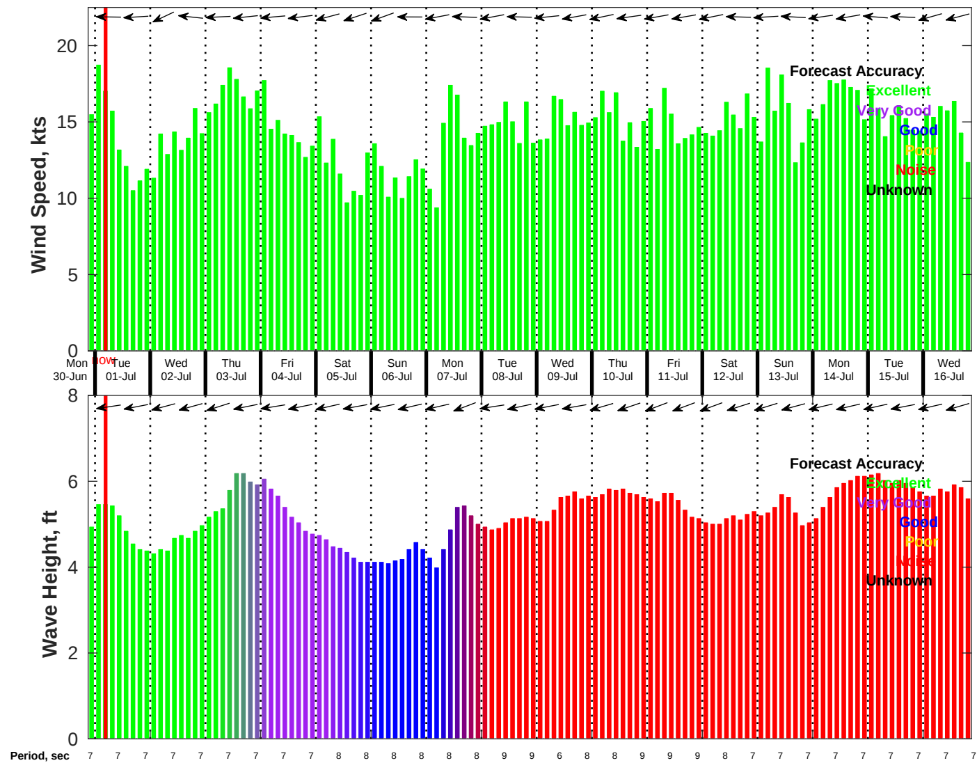
Wind & Wave Forecast for NDBC 41040 from 30-Jun-2025 21:00:00 to 16-Jul-2025 21:00:00
