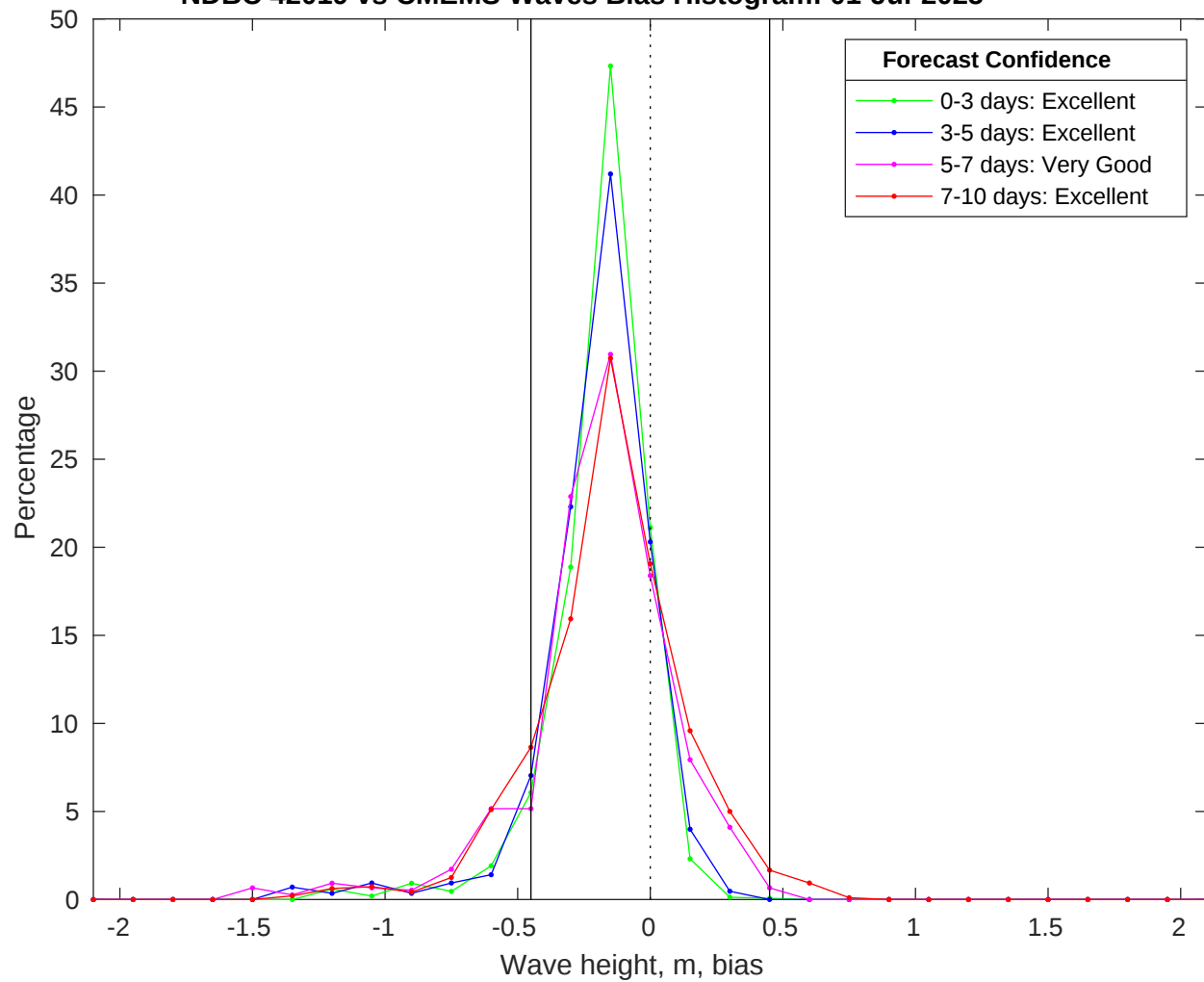
NDBC 42019 vs CMEMS Waves Bias Histogram: 01-Jul-2025
