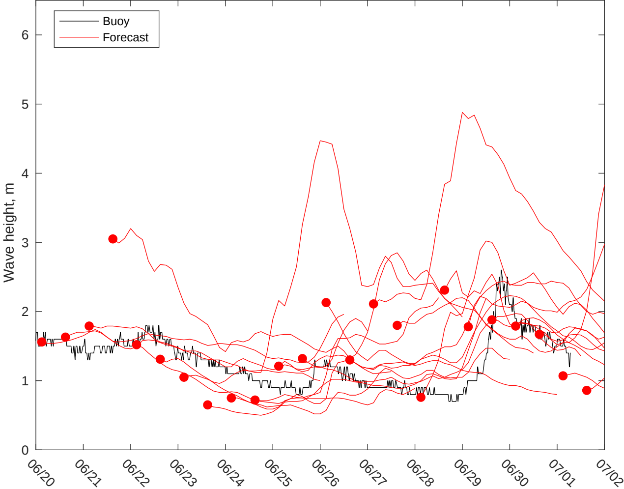
NDBC 42019 vs GFS Waves: 10 to 16 day forecast
