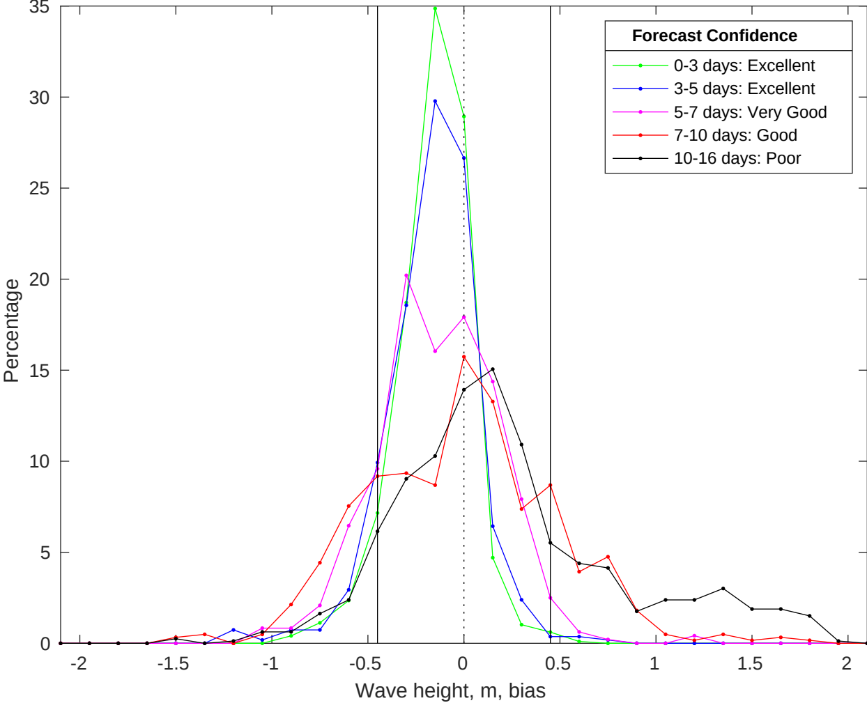
NDBC 42019 vs GFS Waves Bias Histogram: 01-Jul-2025
