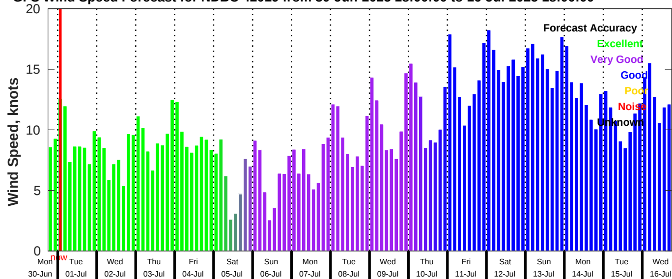
GFS Wind Speed Forecast for NDBC 42019 from 30-Jun-2025 18:00:00 to 16-Jul-2025 18:00:00
