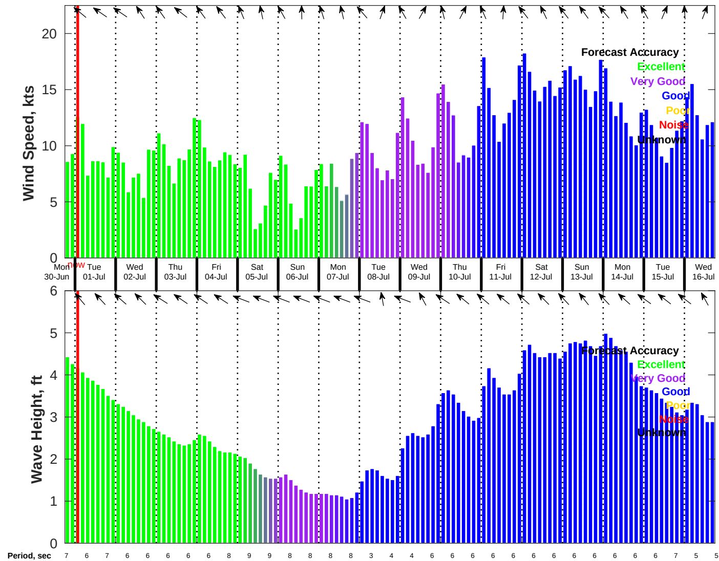
Wind & Wave Forecast for NDBC 42019 from 30-Jun-2025 18:00:00 to 16-Jul-2025 18:00:00
