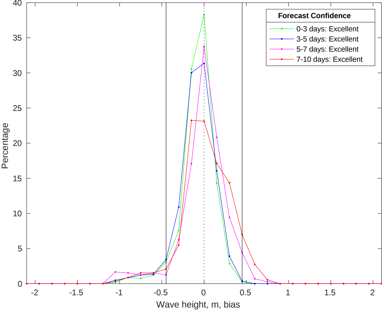
NDBC 42020 vs CMEMS Waves Bias Histogram: 30-Jun-2025
