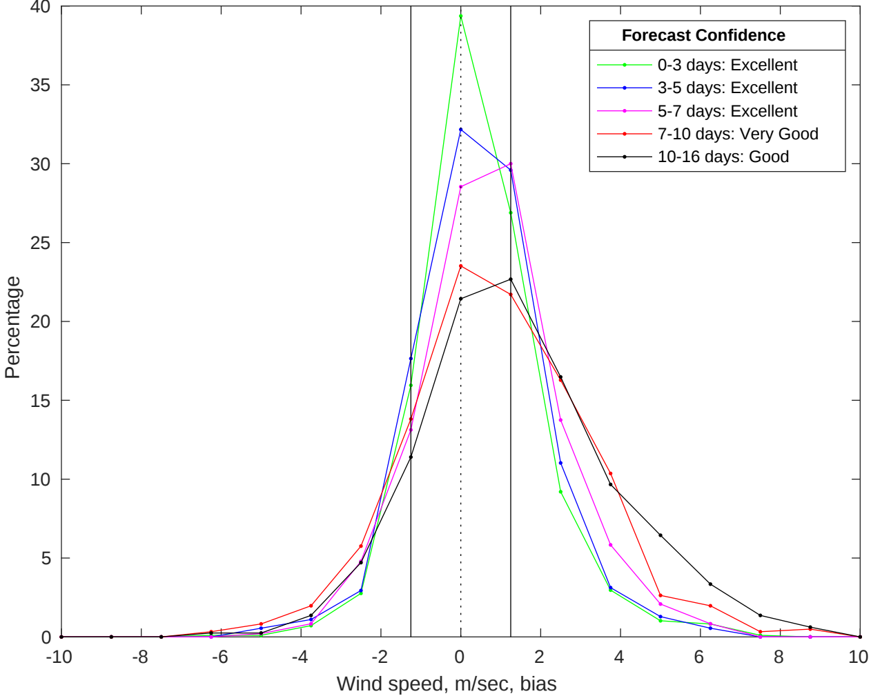
NDBC 42020 vs GFS Winds Bias Histogram: 01-Jul-2025
