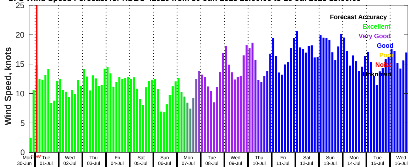
GFS Wind Speed Forecast for NDBC 42020 from 30-Jun-2025 18:00:00 to 16-Jul-2025 18:00:00
