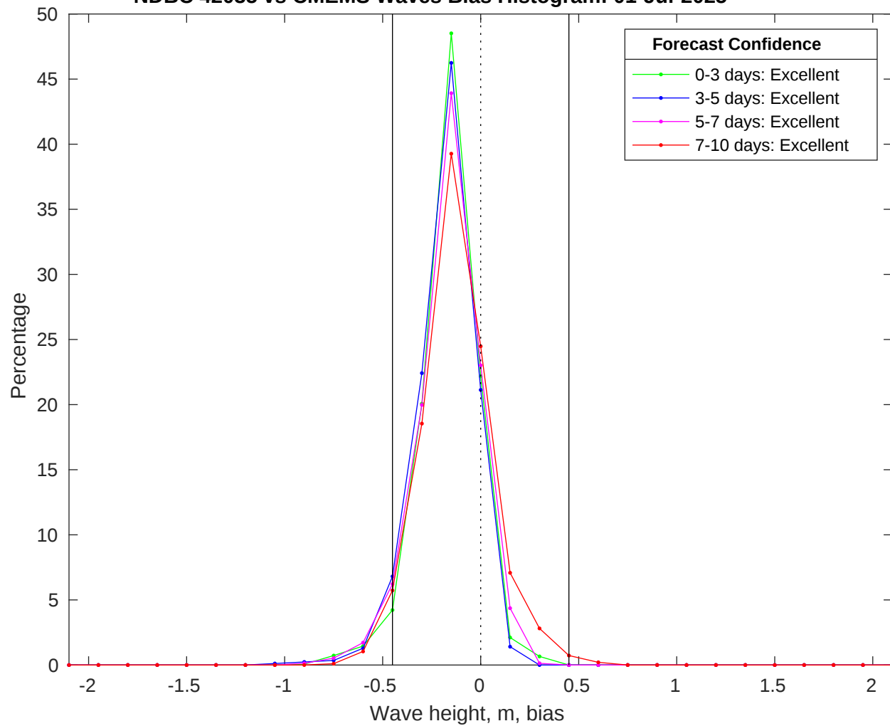
NDBC 42035 vs CMEMS Waves Bias Histogram: 01-Jul-2025
