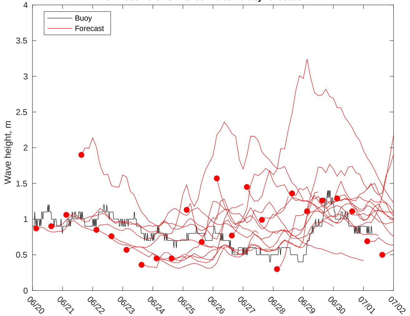
NDBC 42035 vs GFS Waves: 10 to 16 day forecast
