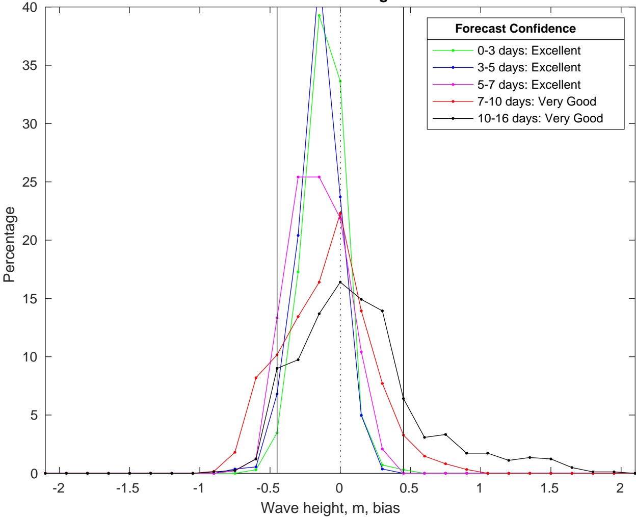
NDBC 42035 vs GFS Waves Bias Histogram: 01-Jul-2025
