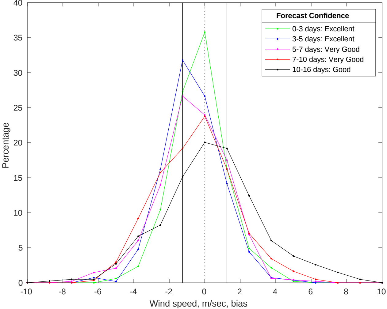
NDBC 42035 vs GFS Winds Bias Histogram: 01-Jul-2025
