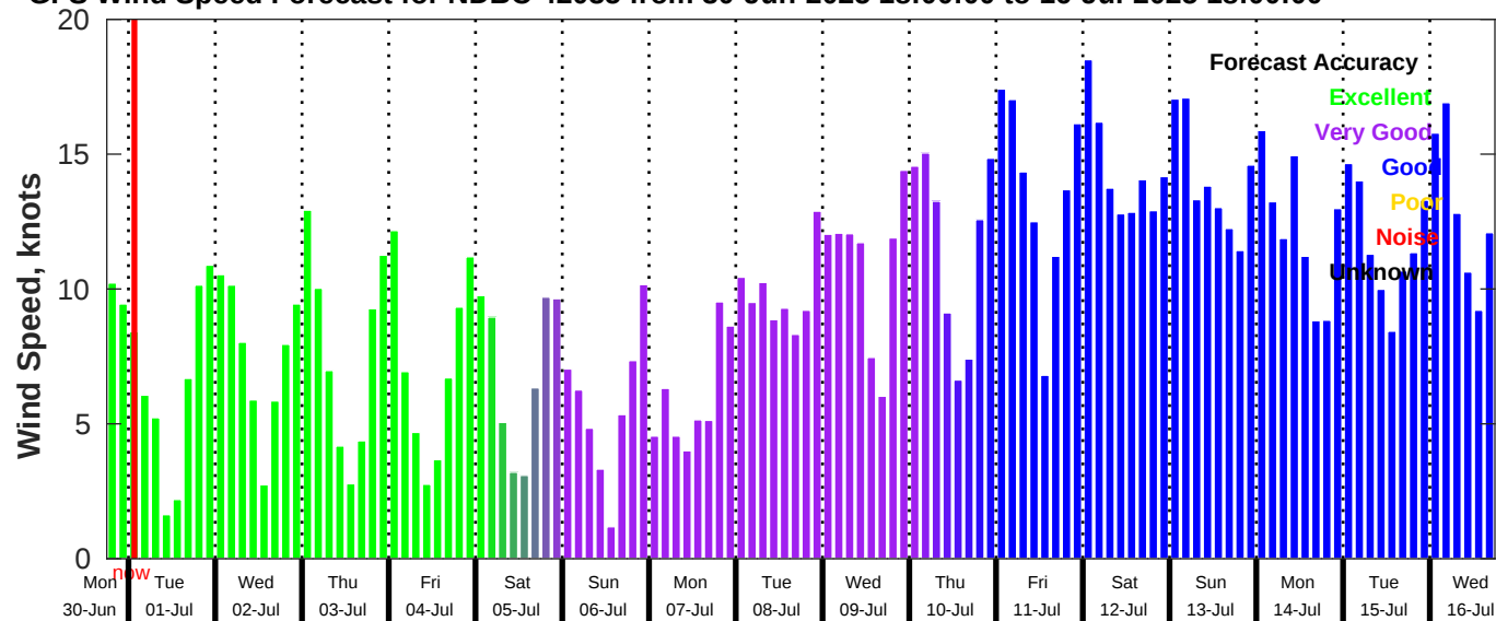
GFS Wind Speed Forecast for NDBC 42035 from 30-Jun-2025 18:00:00 to 16-Jul-2025 18:00:00
