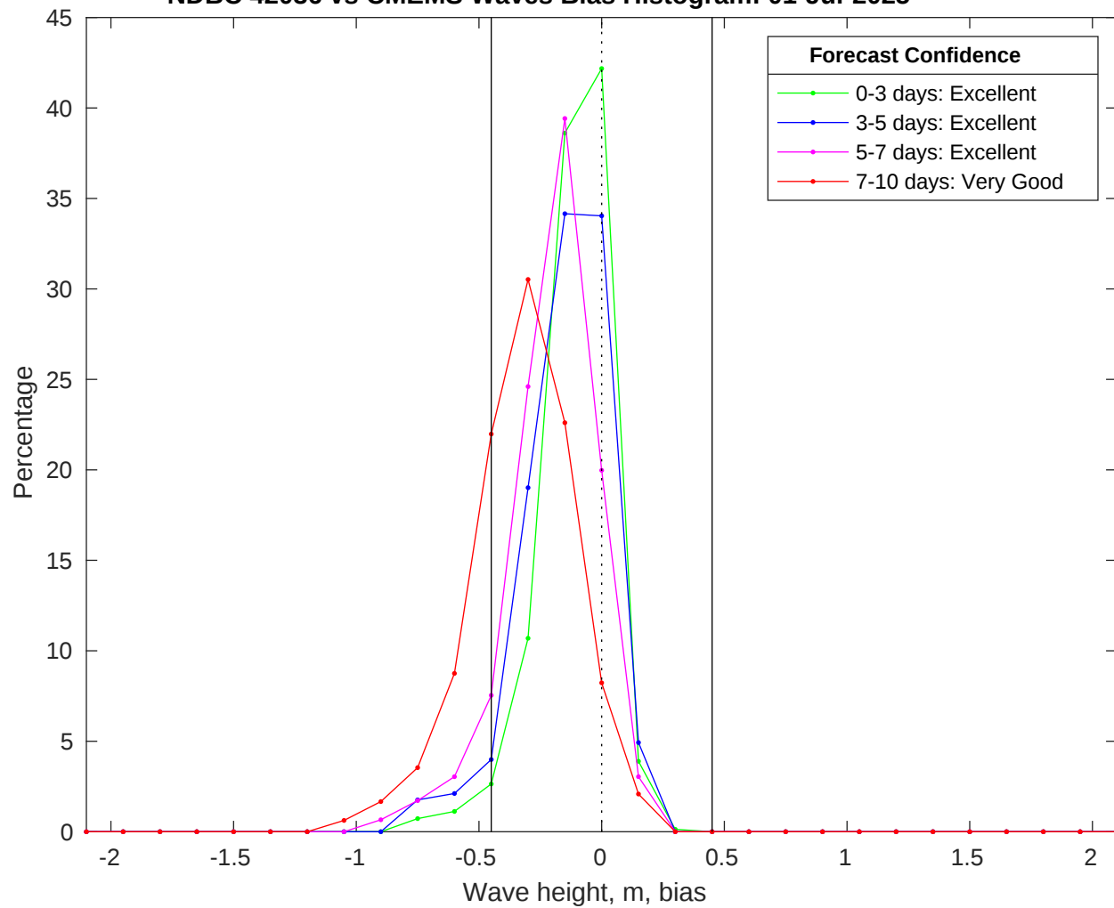
NDBC 42036 vs CMEMS Waves Bias Histogram: 01-Jul-2025
