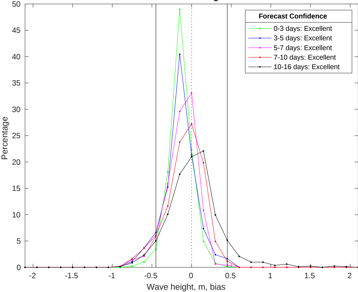
NDBC 42036 vs GFS Waves Bias Histogram: 01-Jul-2025
