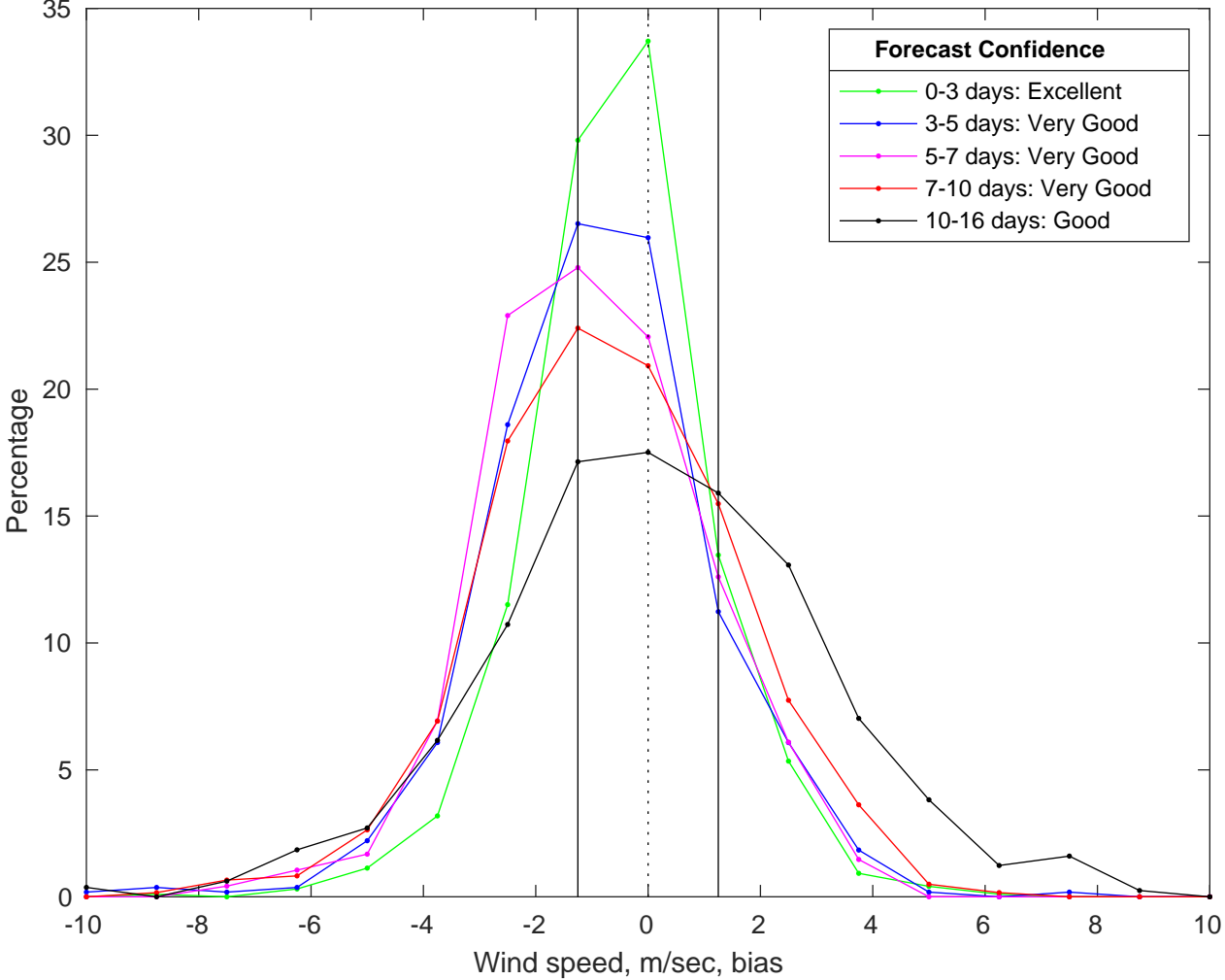
NDBC 42036 vs GFS Winds Bias Histogram: 01-Jul-2025
