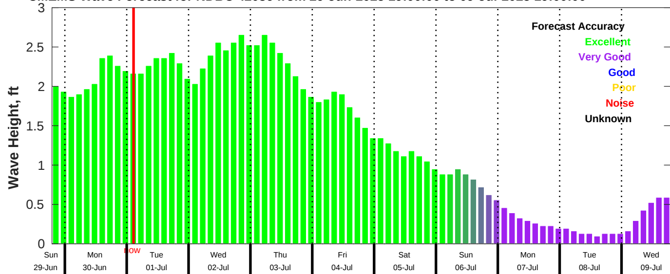
CMEMS Wave Forecast for NDBC 42036 from 29-Jun-2025 19:00:00 to 09-Jul-2025 19:00:00
