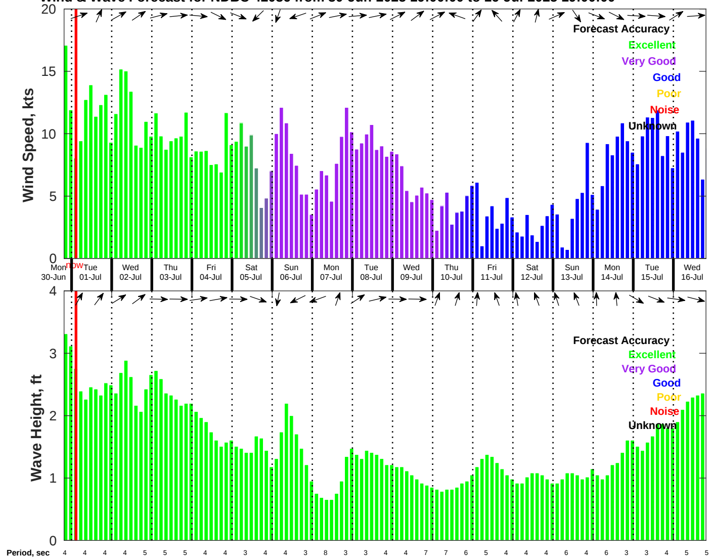
Wind & Wave Forecast for NDBC 42036 from 30-Jun-2025 19:00:00 to 16-Jul-2025 19:00:00
