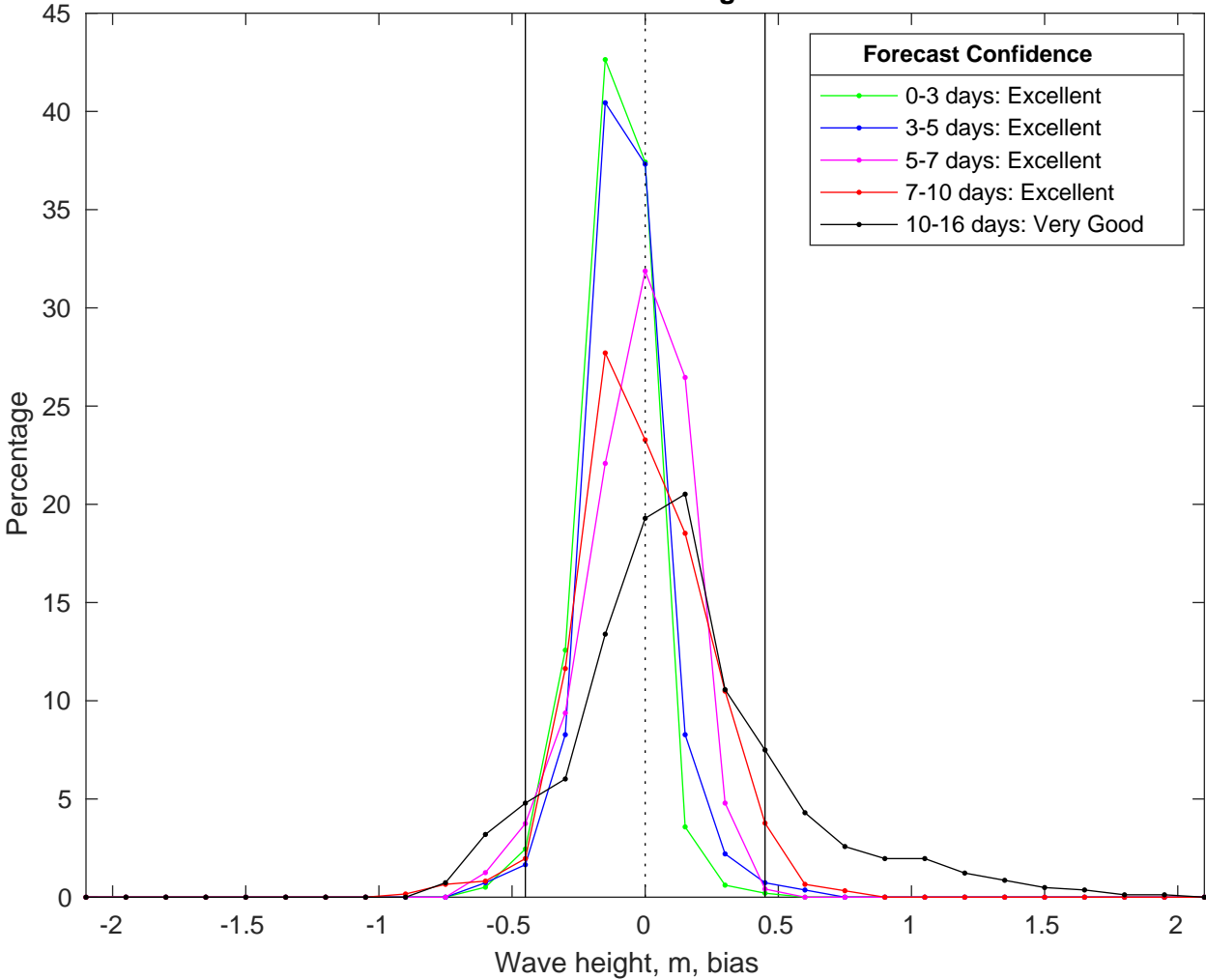
NDBC 42040 vs GFS Waves Bias Histogram: 01-Jul-2025
