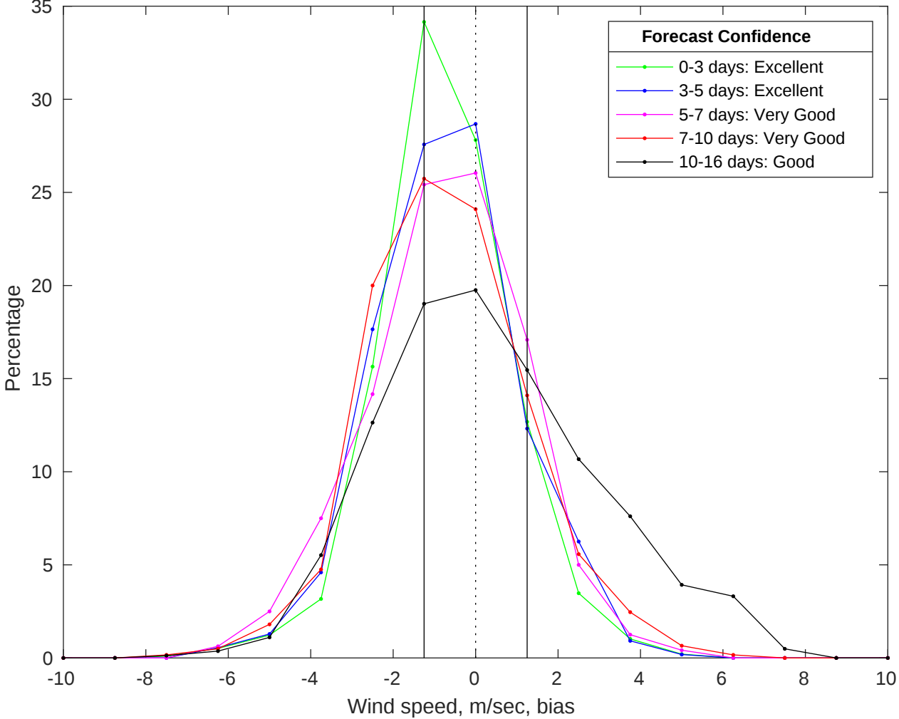
NDBC 42040 vs GFS Winds Bias Histogram: 01-Jul-2025
