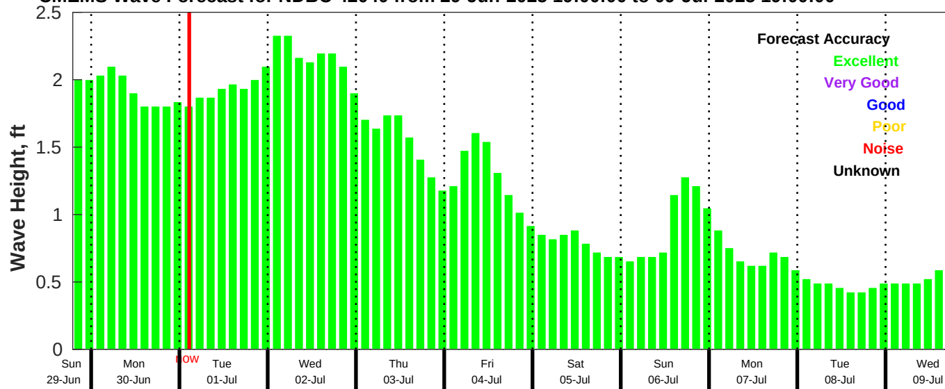
CMEMS Wave Forecast for NDBC 42040 from 29-Jun-2025 19:00:00 to 09-Jul-2025 19:00:00
