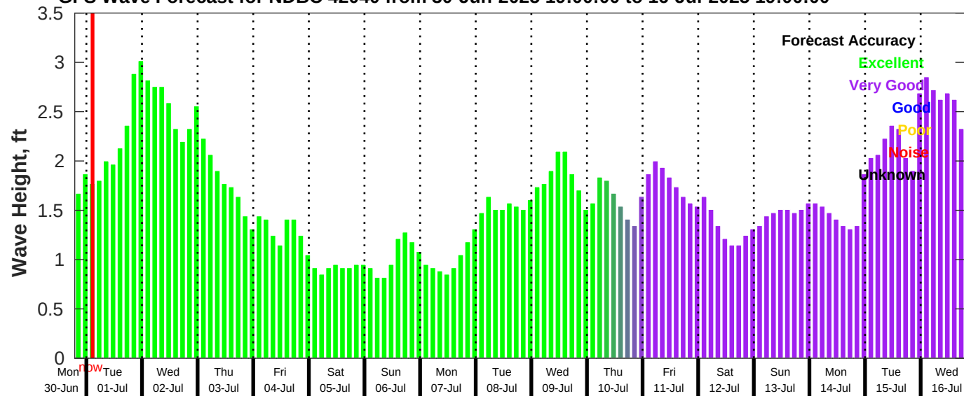
GFS Wave Forecast for NDBC 42040 from 30-Jun-2025 19:00:00 to 16-Jul-2025 19:00:00
