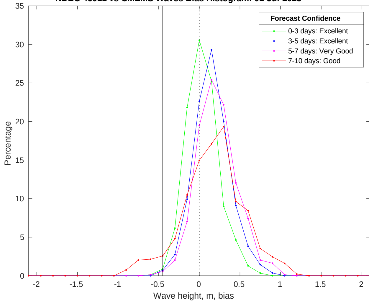
NDBC 46011 vs CMEMS Waves Bias Histogram: 01-Jul-2025
