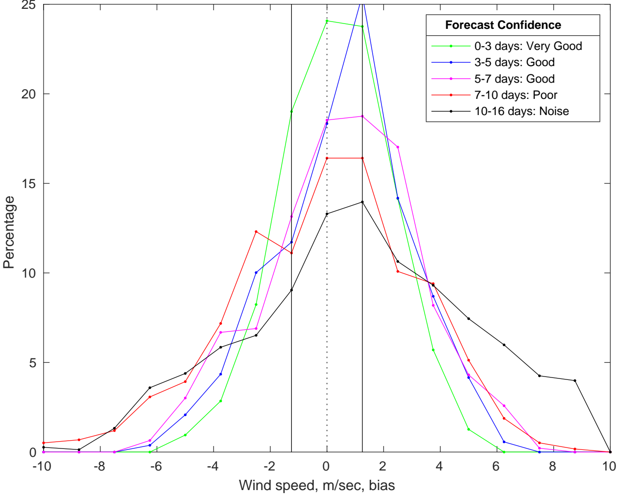
NDBC 46011 vs GFS Winds Bias Histogram: 01-Jul-2025
