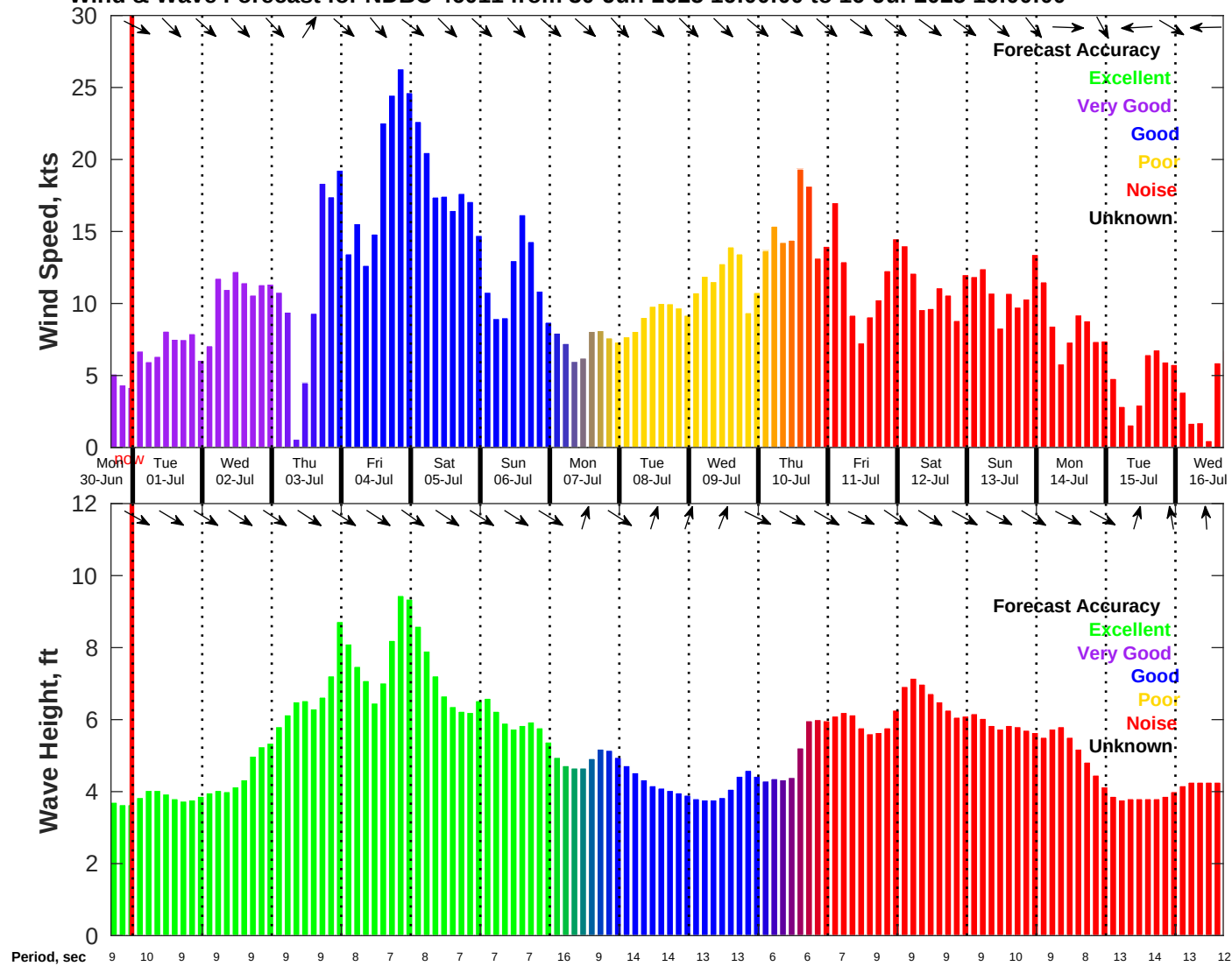
Wind & Wave Forecast for NDBC 46011 from 30-Jun-2025 16:00:00 to 16-Jul-2025 16:00:00
