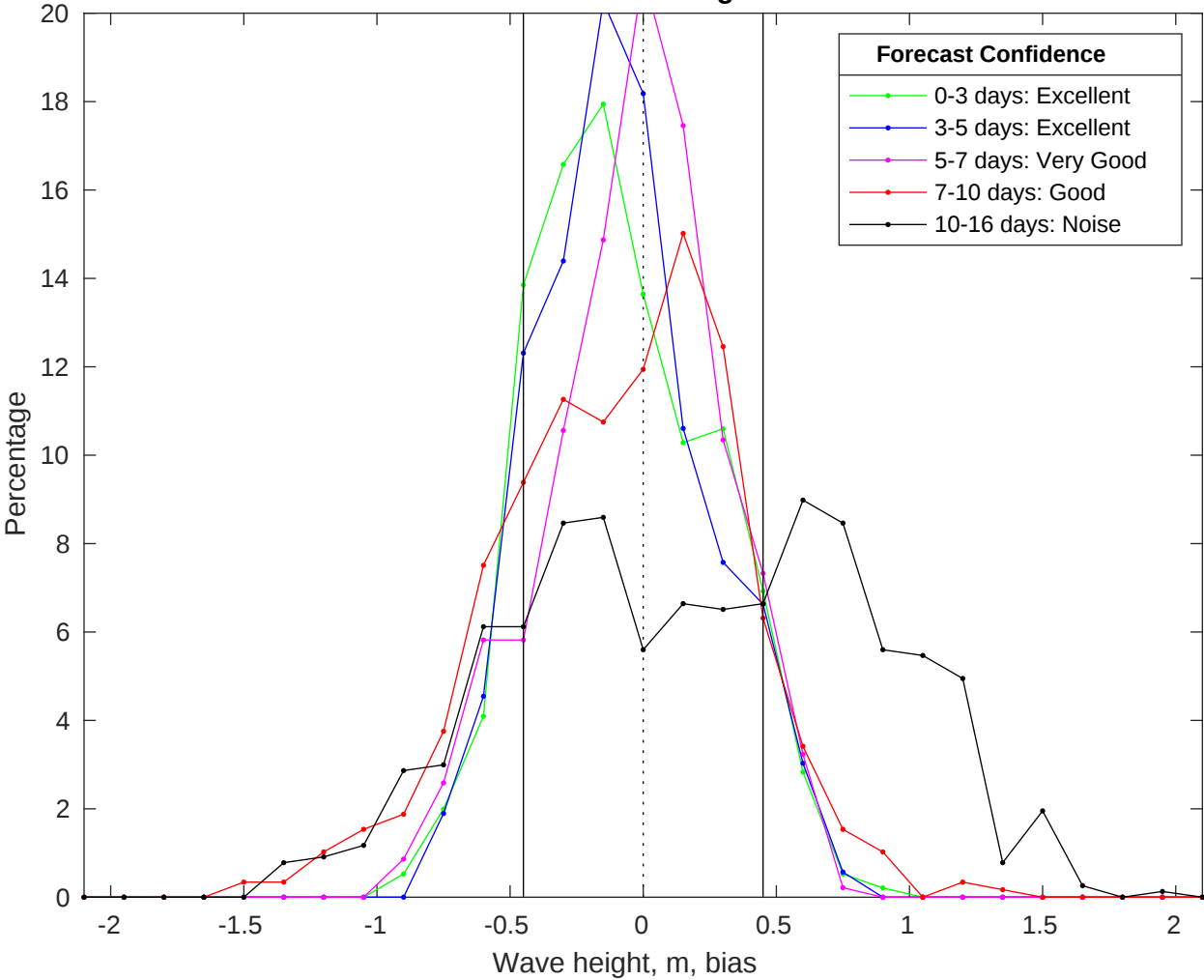
NDBC 46028 vs GFS Waves Bias Histogram: 01-Jul-2025
