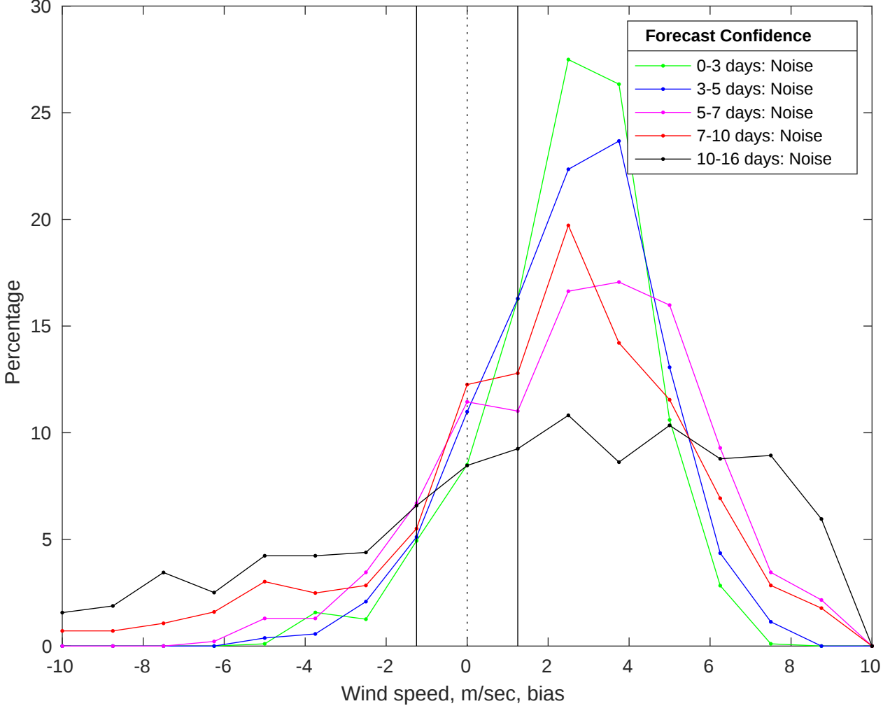
NDBC 46028 vs GFS Winds Bias Histogram: 01-Jul-2025
