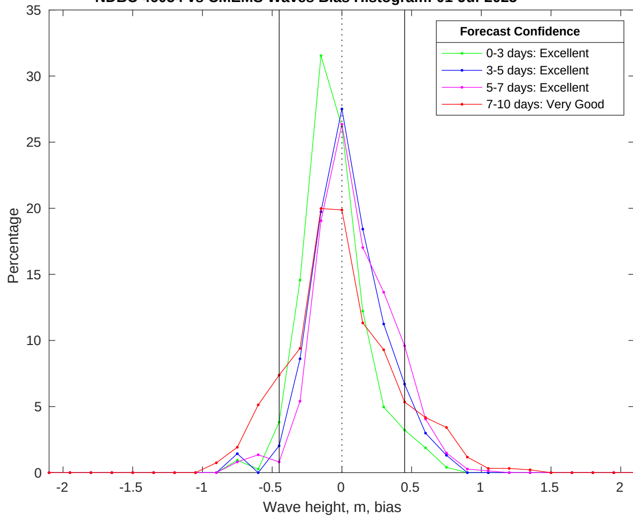
NDBC 46054 vs CMEMS Waves Bias Histogram: 01-Jul-2025
