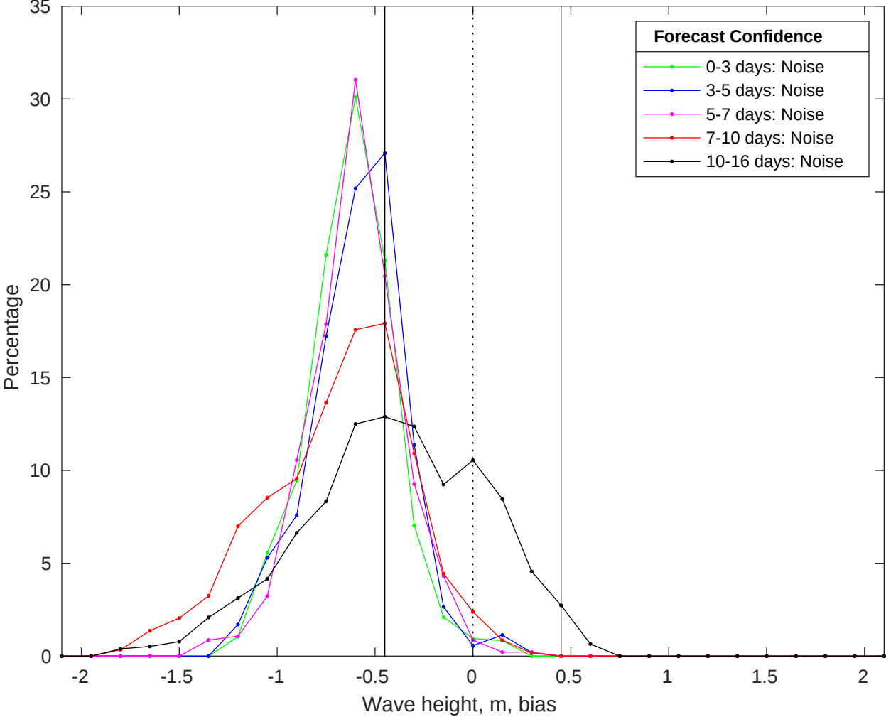
NDBC 46054 vs GFS Waves Bias Histogram: 01-Jul-2025
