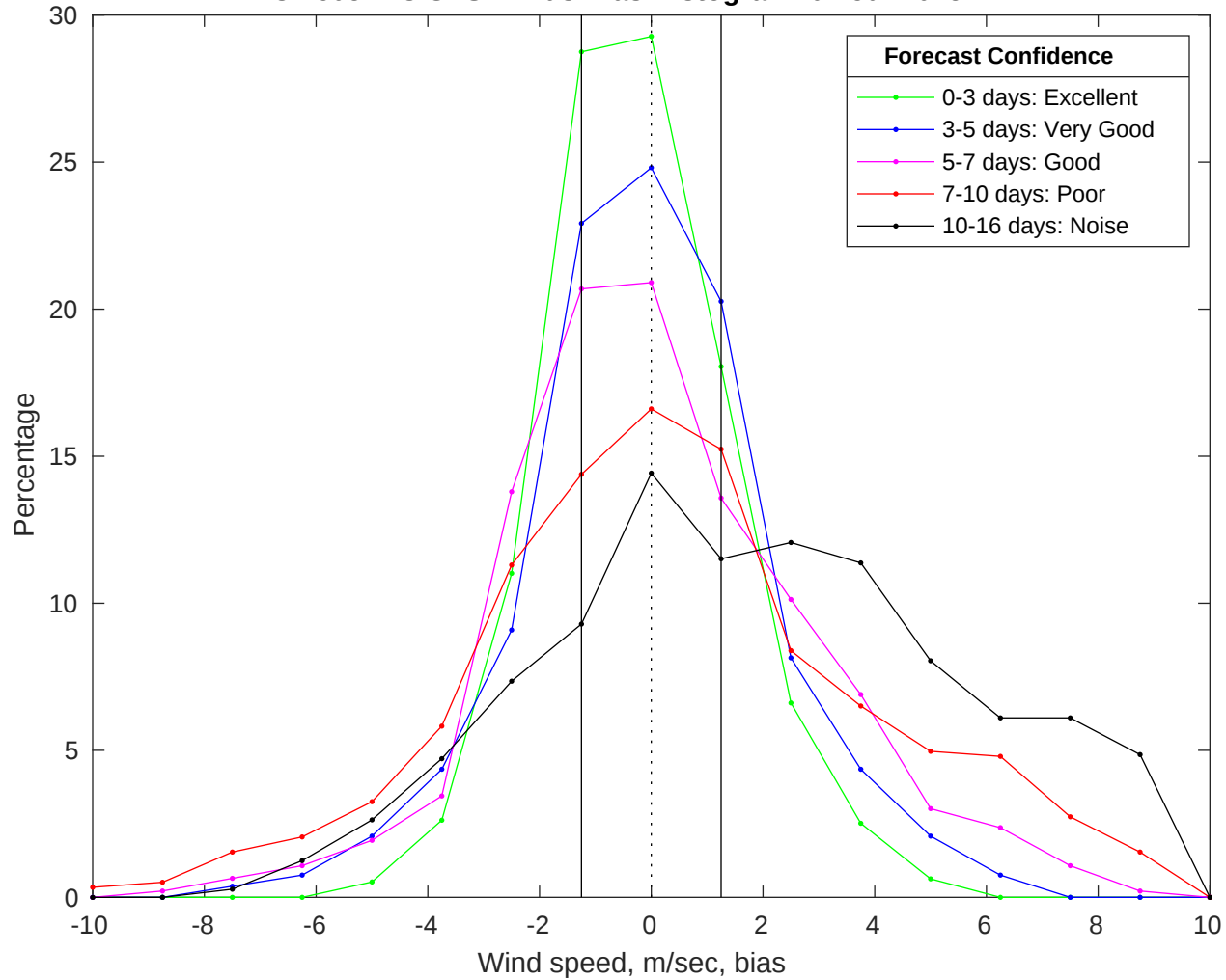
NDBC 46054 vs GFS Winds Bias Histogram: 01-Jul-2025
