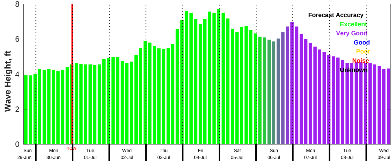
CMEMS Wave Forecast for NDBC 46054 from 29-Jun-2025 16:00:00 to 09-Jul-2025 16:00:00
