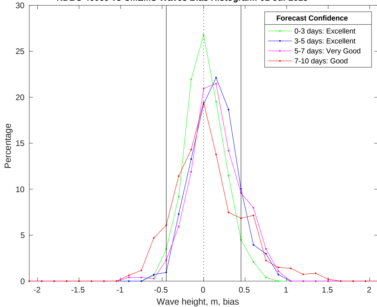
NDBC 46069 vs CMEMS Waves Bias Histogram: 01-Jul-2025
