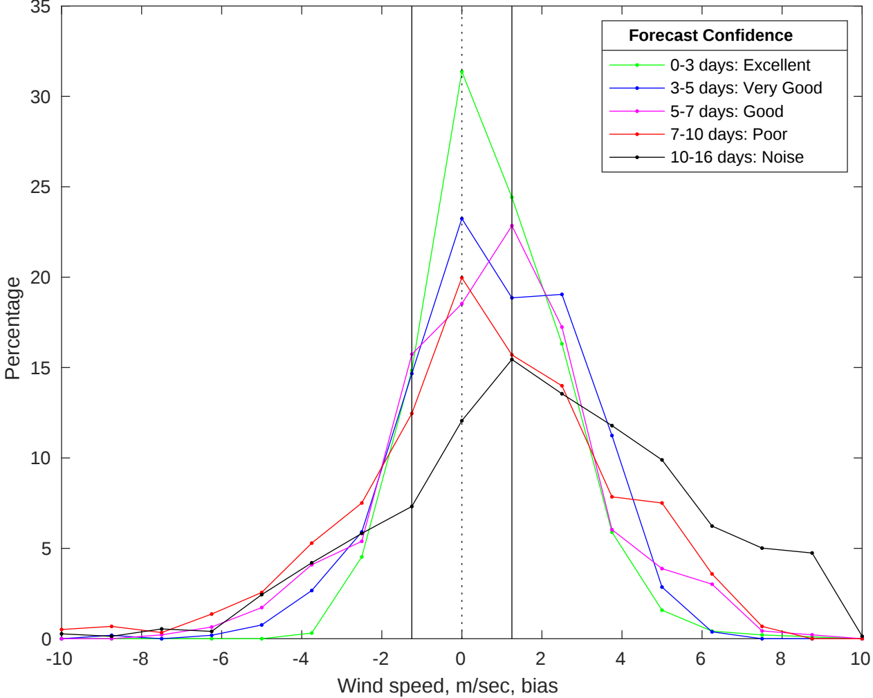
NDBC 46069 vs GFS Winds Bias Histogram: 01-Jul-2025
