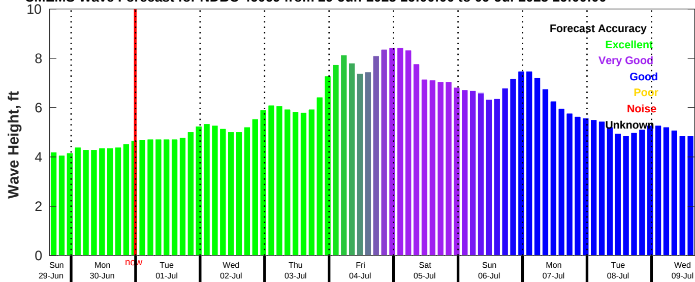
CMEMS Wave Forecast for NDBC 46069 from 29-Jun-2025 16:00:00 to 09-Jul-2025 16:00:00
