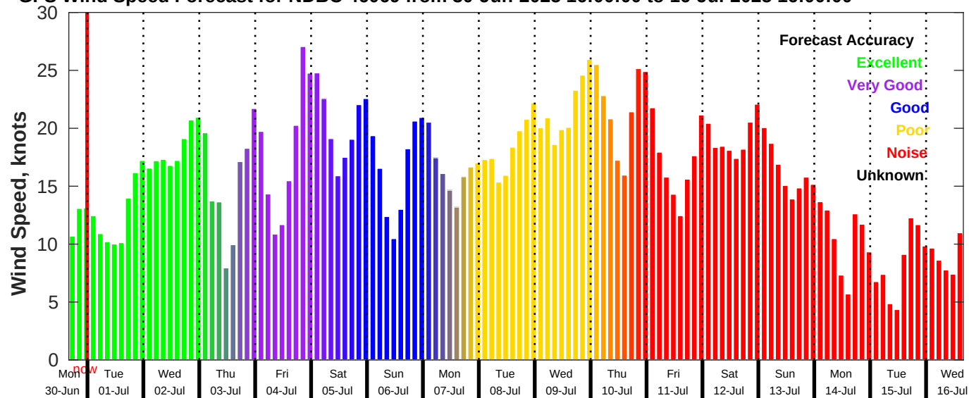
GFS Wind Speed Forecast for NDBC 46069 from 30-Jun-2025 16:00:00 to 16-Jul-2025 16:00:00
