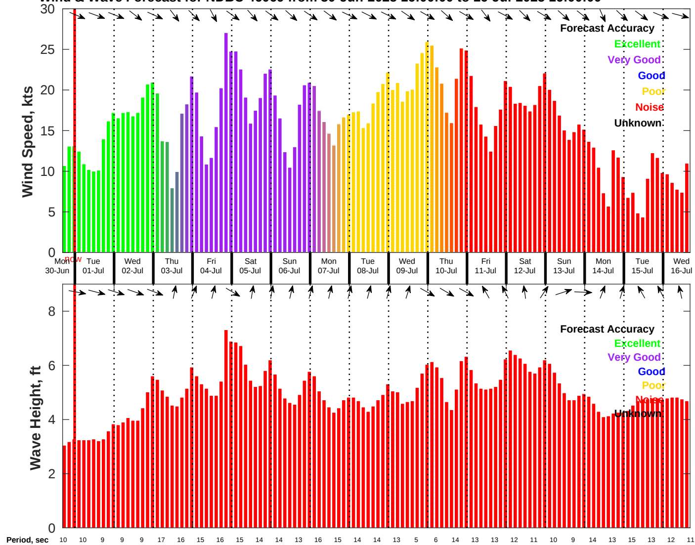
Wind & Wave Forecast for NDBC 46069 from 30-Jun-2025 16:00:00 to 16-Jul-2025 16:00:00
