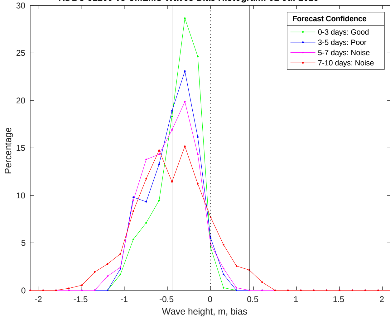
NDBC 51209 vs CMEMS Waves Bias Histogram: 01-Jul-2025
