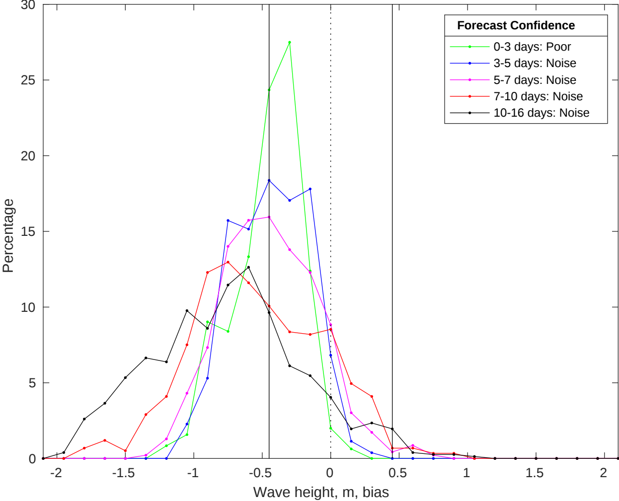
NDBC 51209 vs GFS Waves Bias Histogram: 01-Jul-2025
