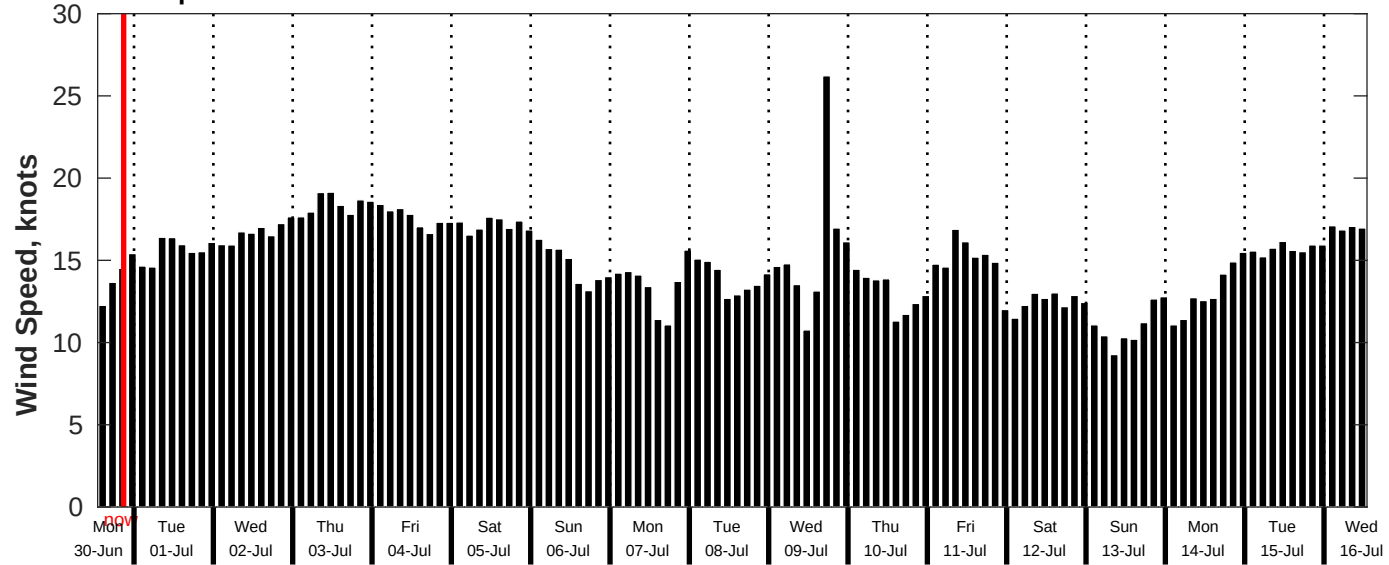
GFS Wind Speed Forecast for NDBC 51209 from 30-Jun-2025 13:00:00 to 16-Jul-2025 13:00:00
