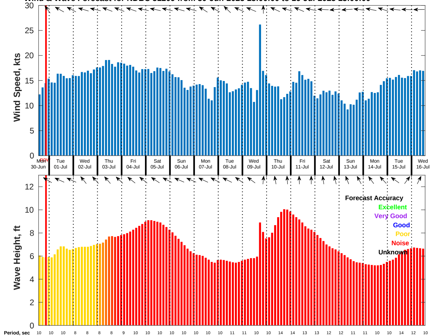
Wind & Wave Forecast for NDBC 51209 from 30-Jun-2025 13:00:00 to 16-Jul-2025 13:00:00
