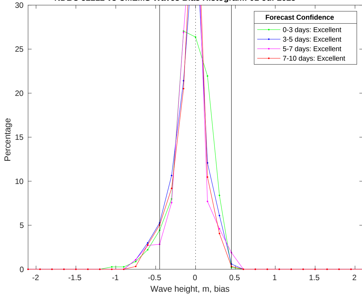
NDBC 52212 vs CMEMS Waves Bias Histogram: 01-Jul-2025
