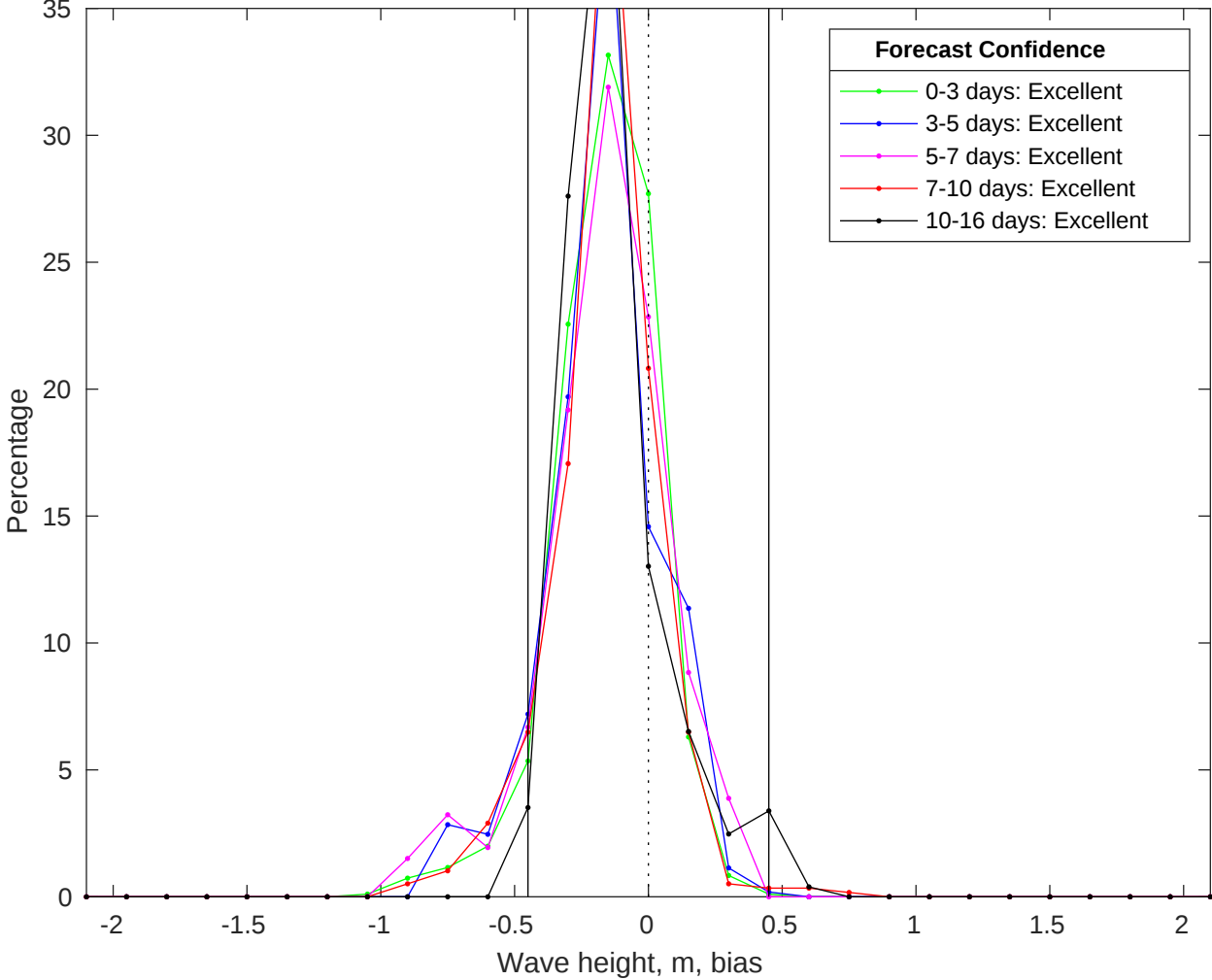
NDBC 52212 vs GFS Waves Bias Histogram: 01-Jul-2025
